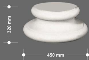
BB-C 300B Width:Ø450mm × Height:320mm
